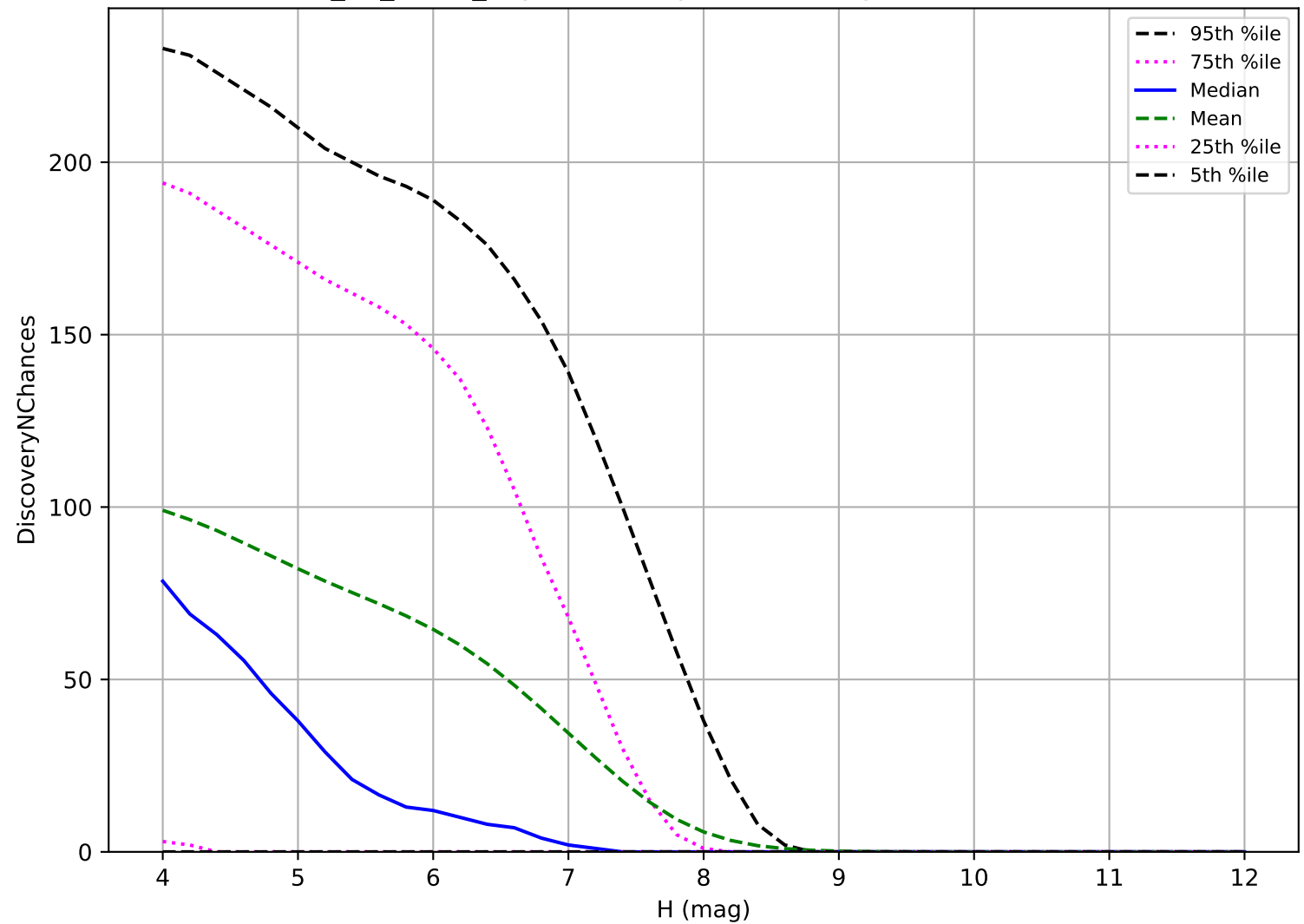
too_10_1v3.4_10yrs: TNO 3 pairs in 15 nights detection loss
