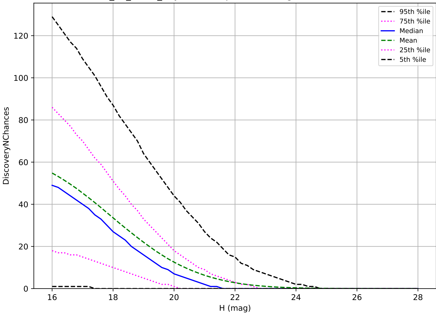
too_10_1v3.4_10yrs: PHA 3 pairs in 15 nights detection loss
