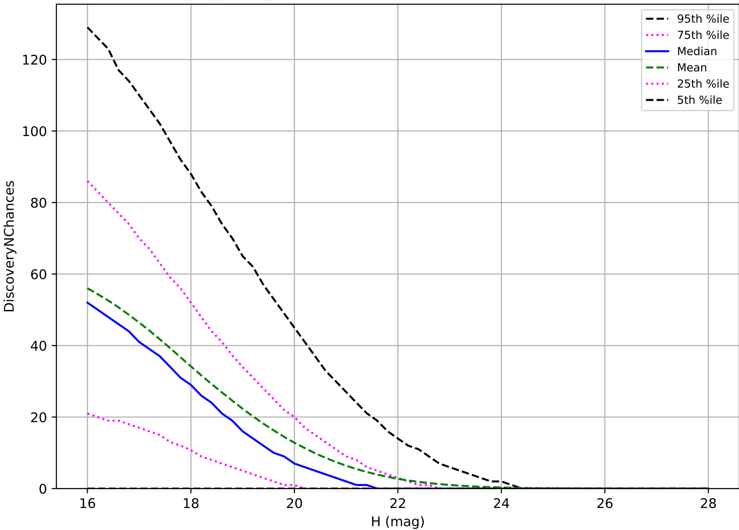
too_10_1v3.4_10yrs: NEO 3 pairs in 15 nights detection loss
