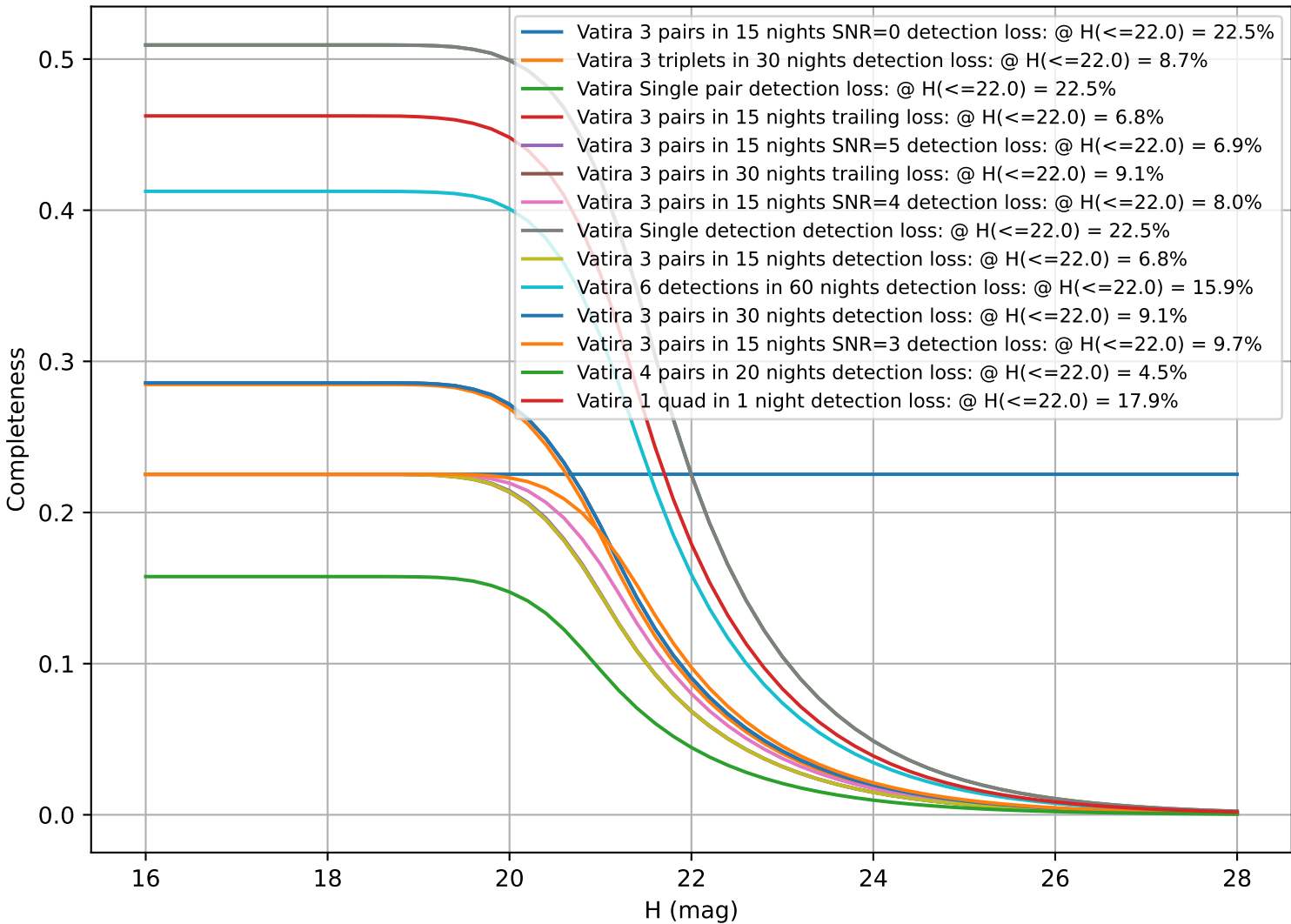
too_10_1v3.4_10yrs: CumulativeCompleteness
