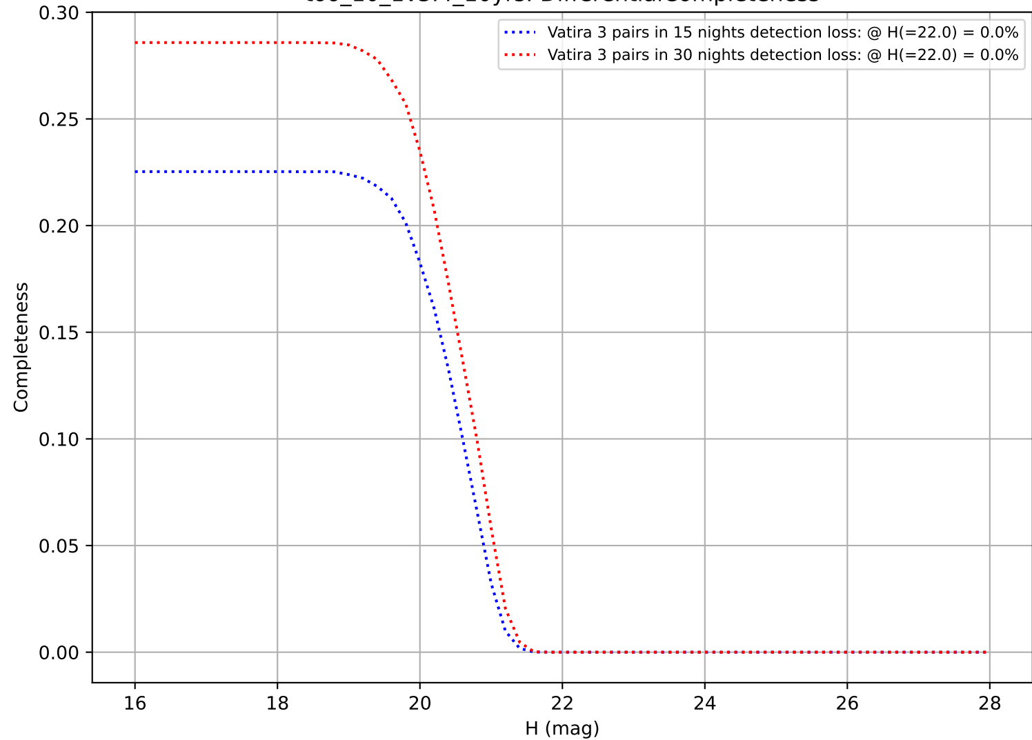
too_10_1v3.4_10yrs: DifferentialCompleteness
