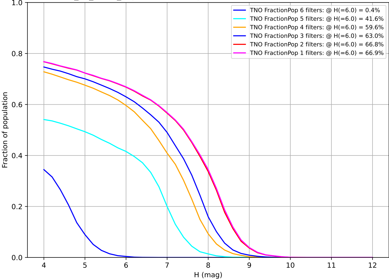
too_10_1v3.4_10yrs: Fraction of population with colors in X filters TNO
