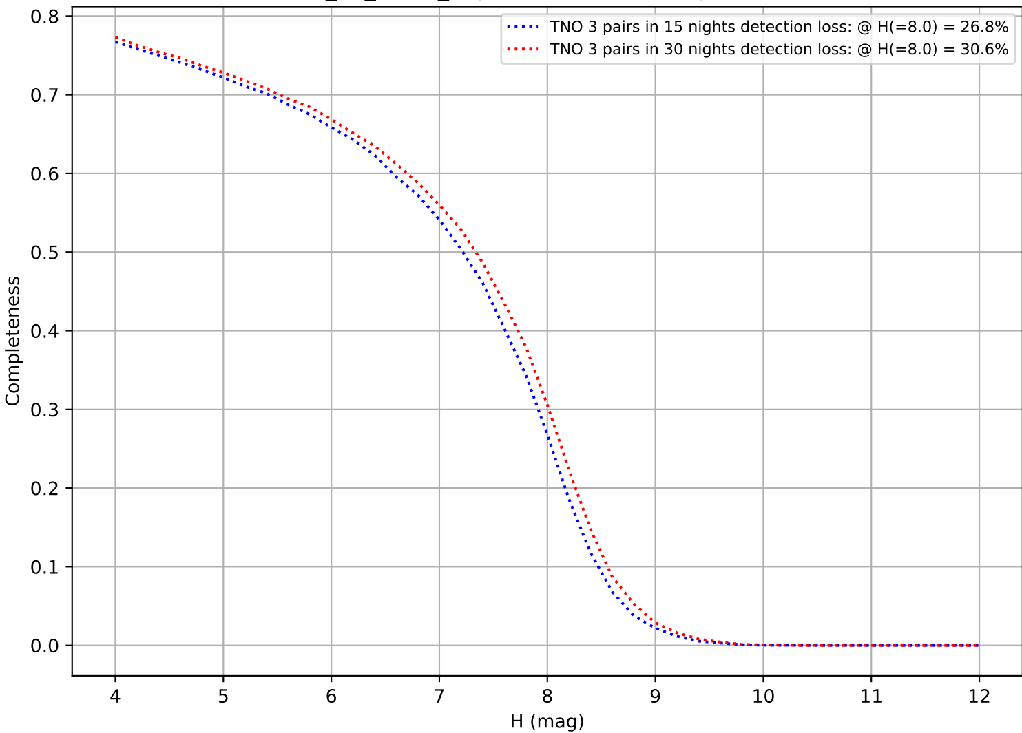
too_10_1v3.4_10yrs: DifferentialCompleteness
