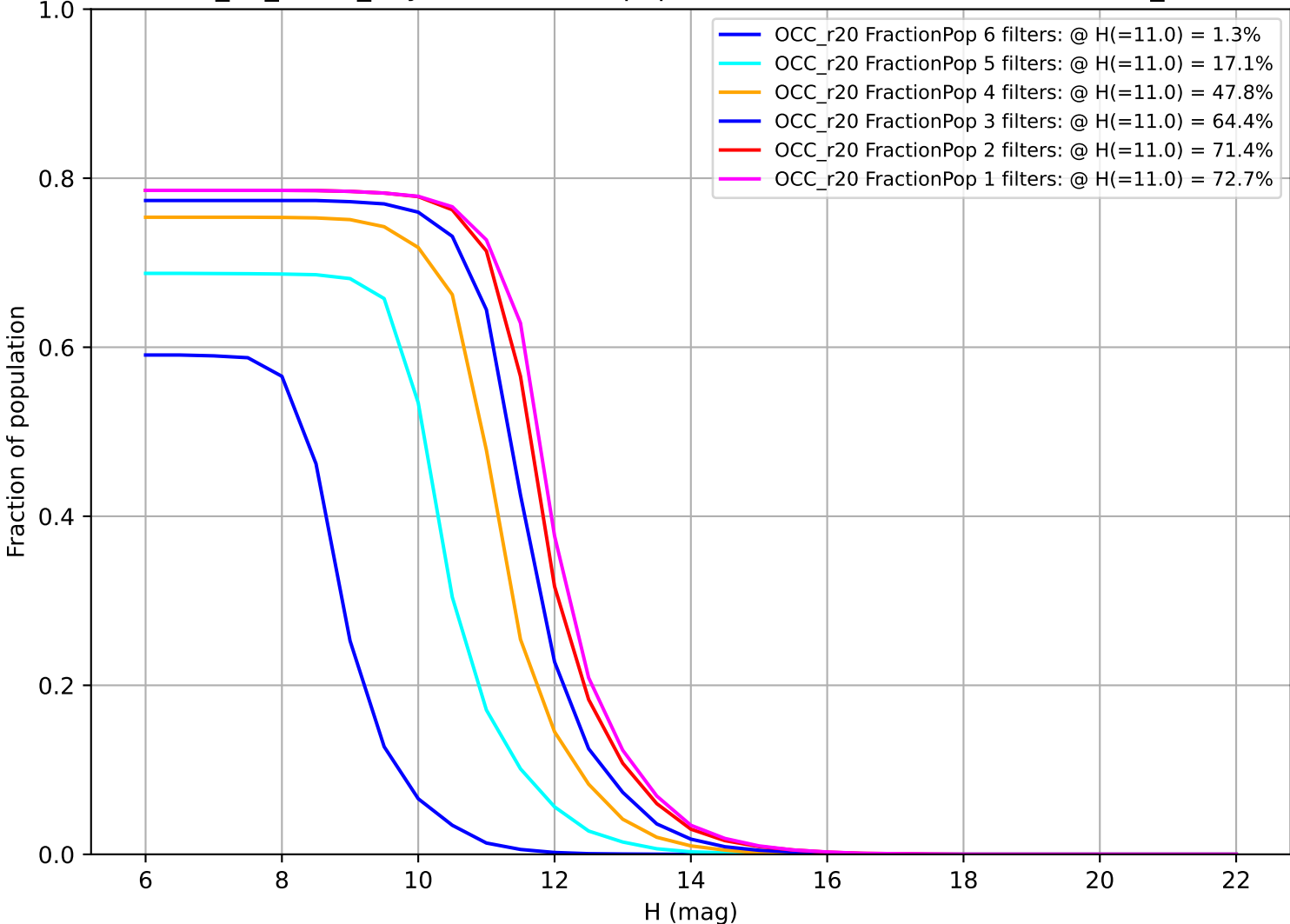
too_10_1v3.4_10yrs: Fraction of population with colors in X filters OCC_r20
