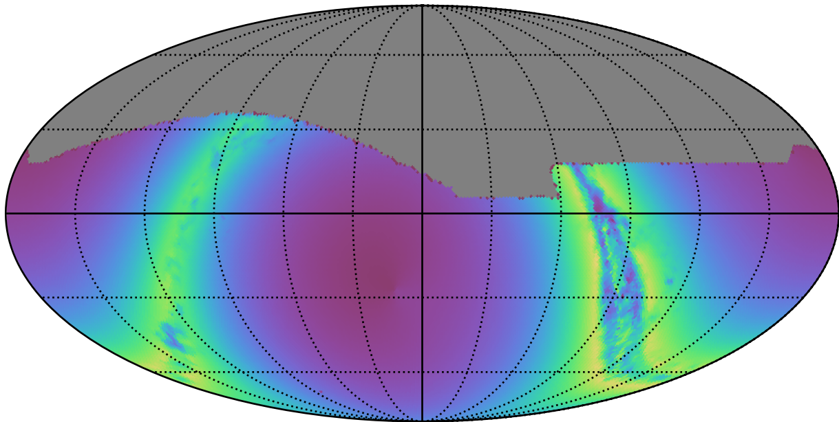
too_10_1v3.4_10yrs : young_stars
