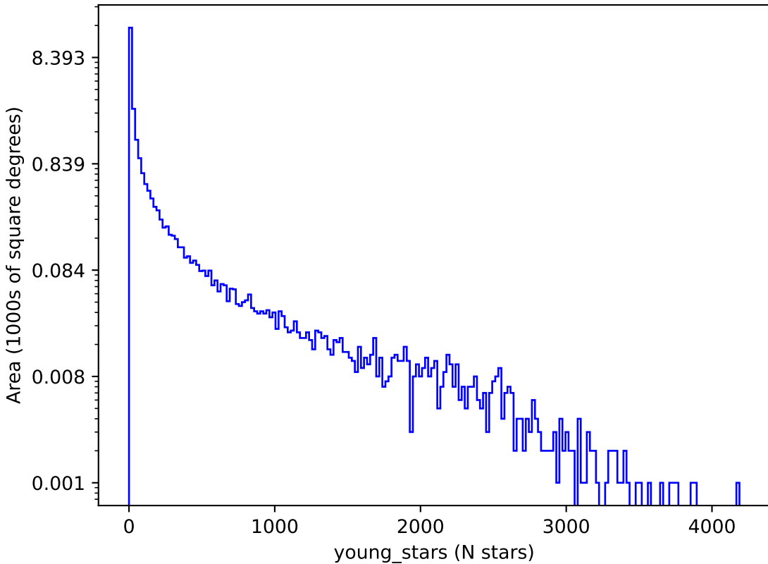
too_10_1v3.4_10yrs : young_stars
