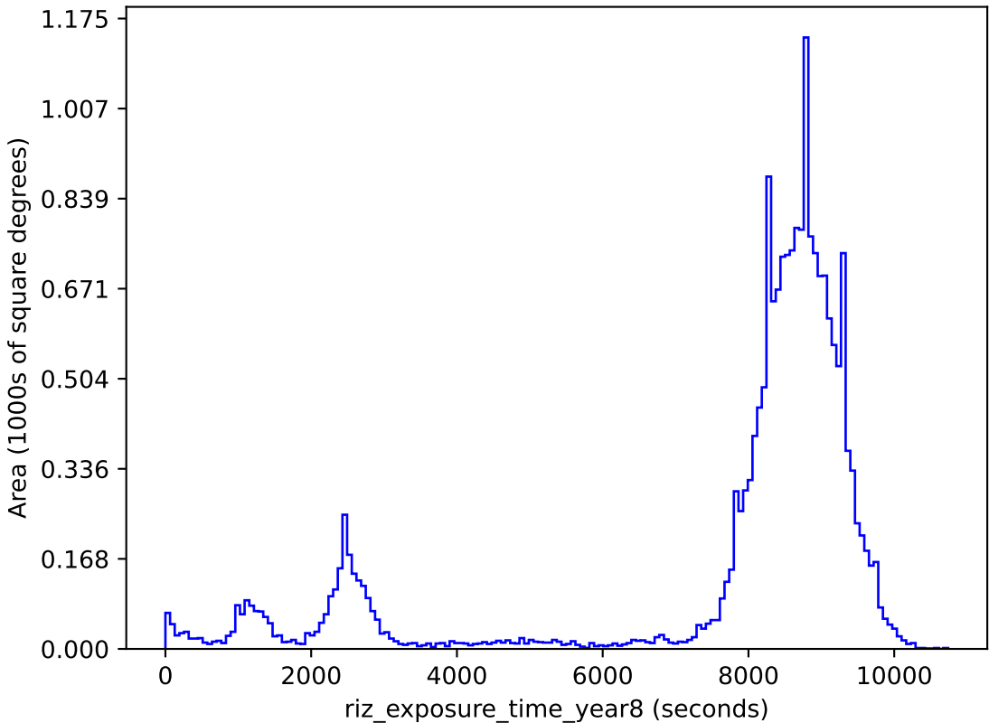
too_10_1v3.4_10yrs gri band non-DD: riz_exposure_time_year8
