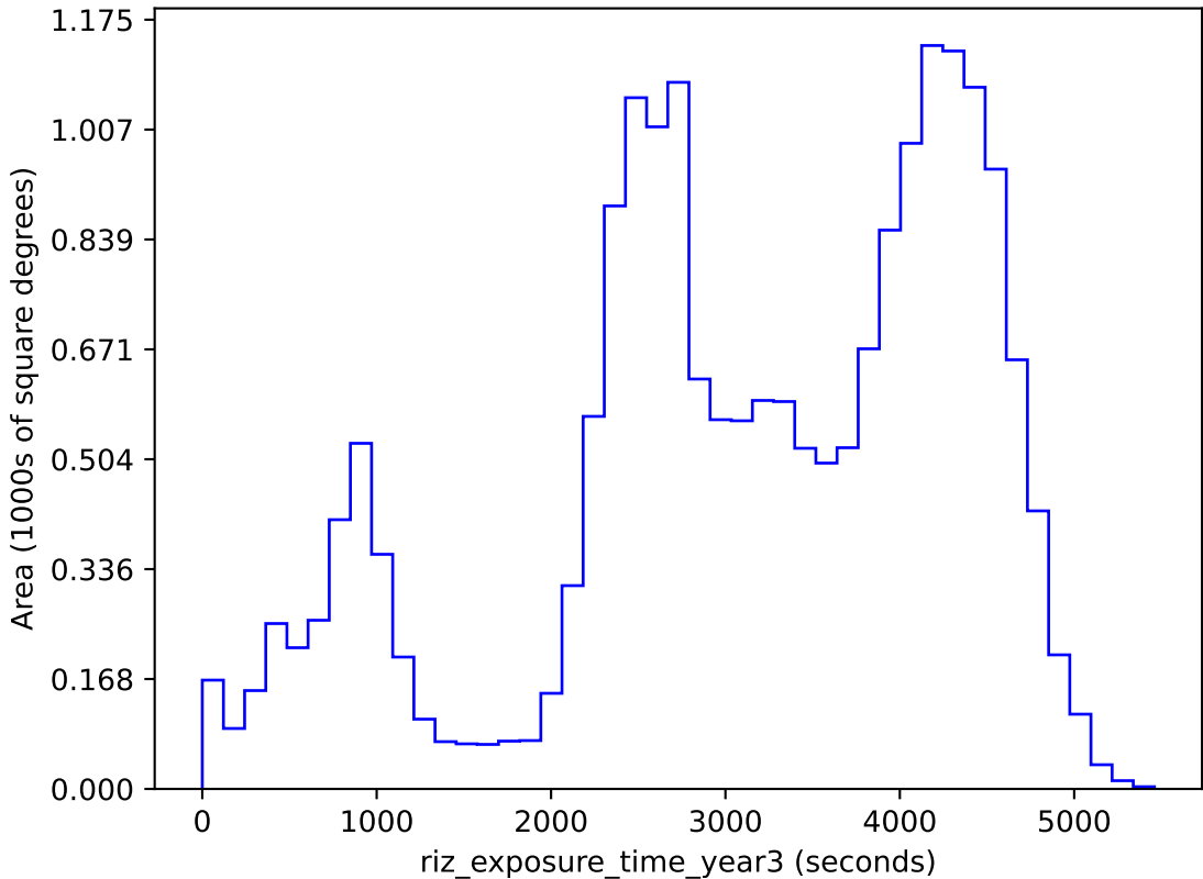
too_10_1v3.4_10yrs gri band non-DD: riz_exposure_time_year3
