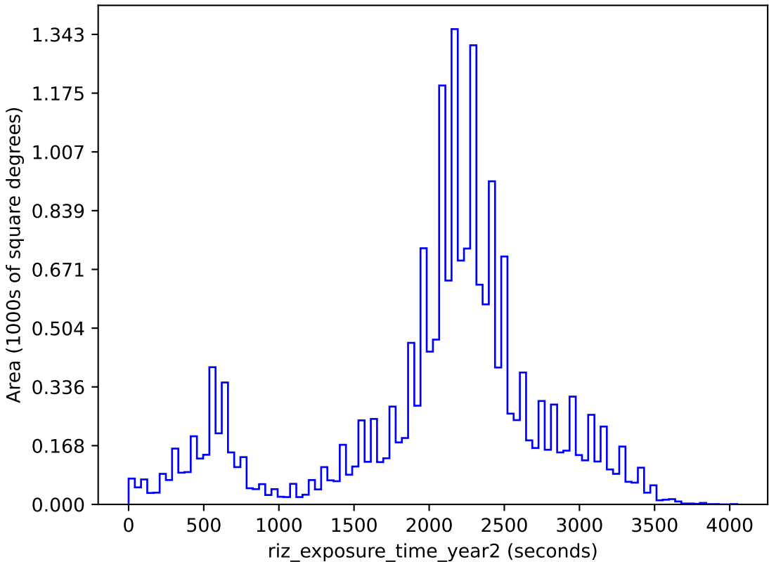
too_10_1v3.4_10yrs gri band non-DD: riz_exposure_time_year2
