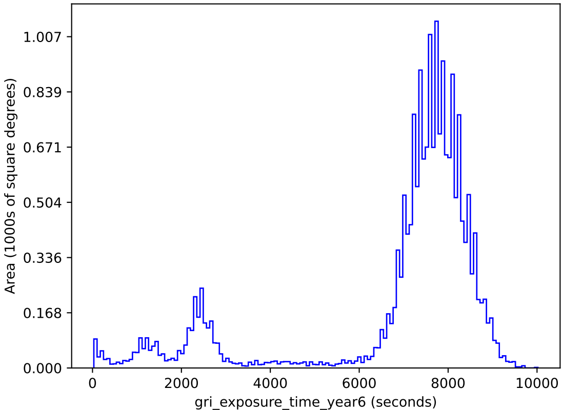
too_10_1v3.4_10yrs gri band non-DD: gri_exposure_time_year6
