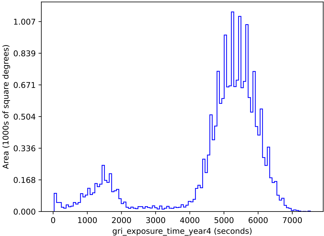
too_10_1v3.4_10yrs gri band non-DD: gri_exposure_time_year4
