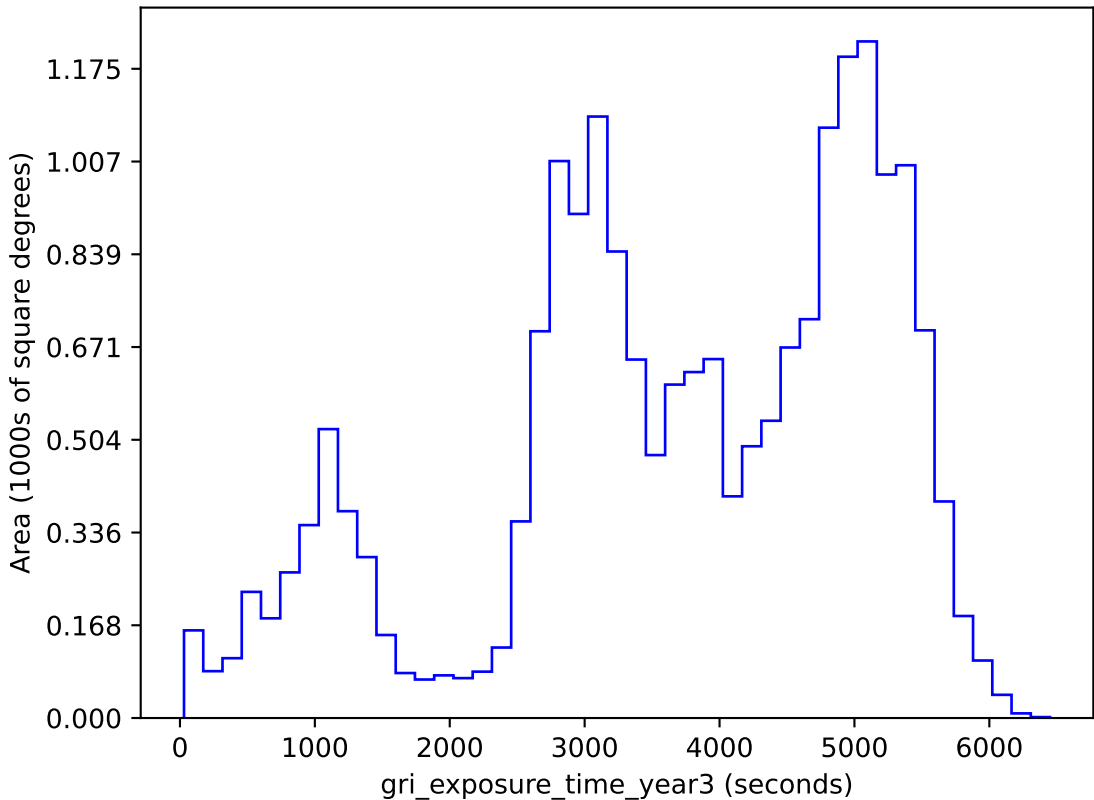
too_10_1v3.4_10yrs gri band non-DD: gri_exposure_time_year3
