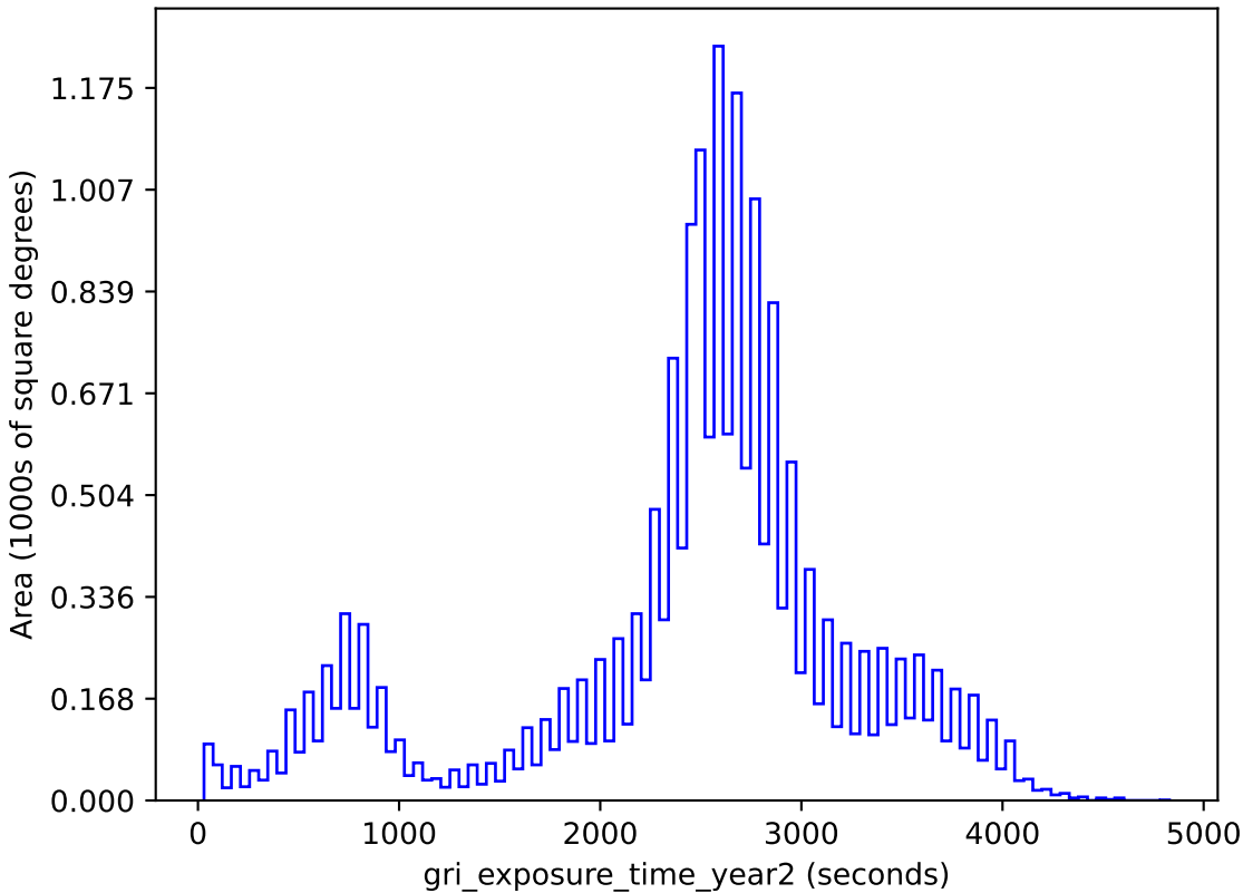
too_10_1v3.4_10yrs gri band non-DD: gri_exposure_time_year2
