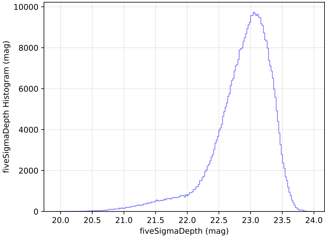
too_10_1v3.4_10yrs z: fiveSigmaDepth Histogram
