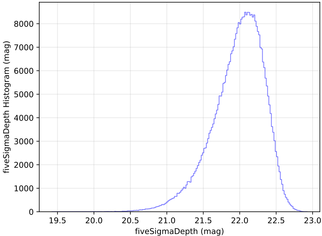
too_10_1v3.4_10yrs y: fiveSigmaDepth Histogram
