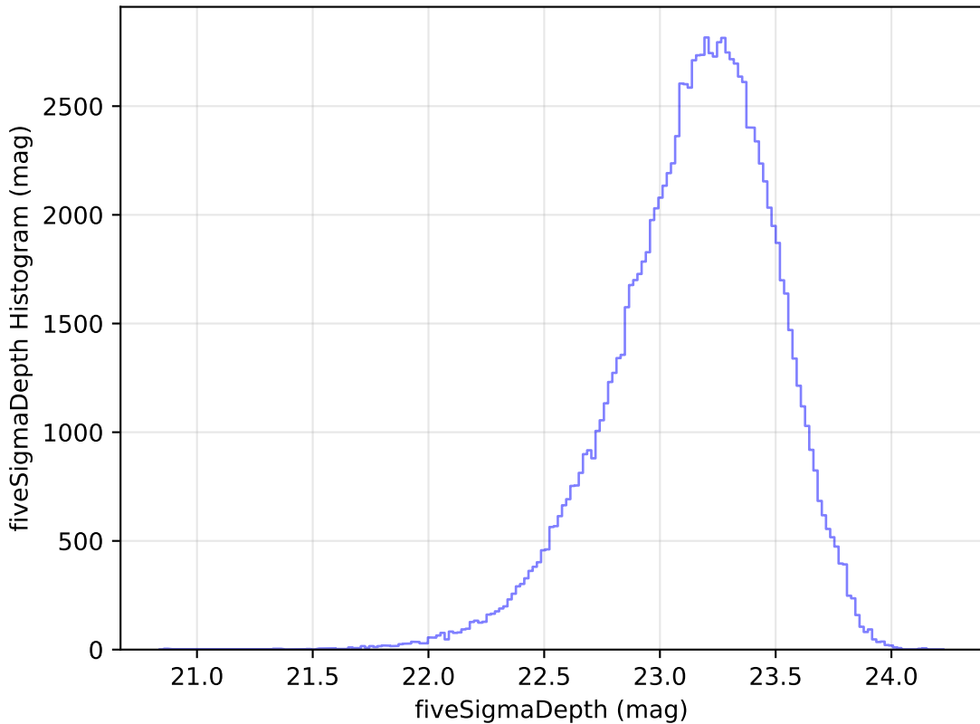
too_10_1v3.4_10yrs u: fiveSigmaDepth Histogram
