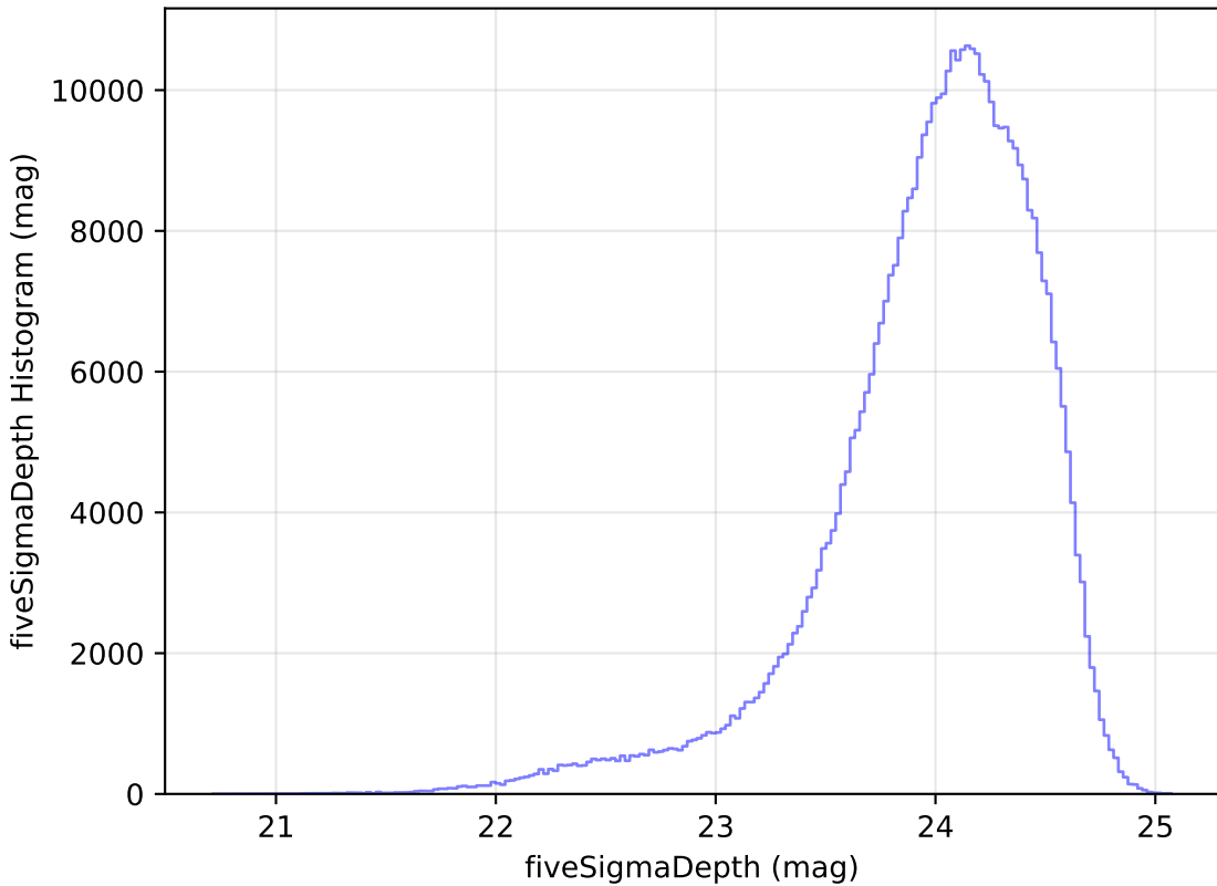
too_10_1v3.4_10yrs r: fiveSigmaDepth Histogram
