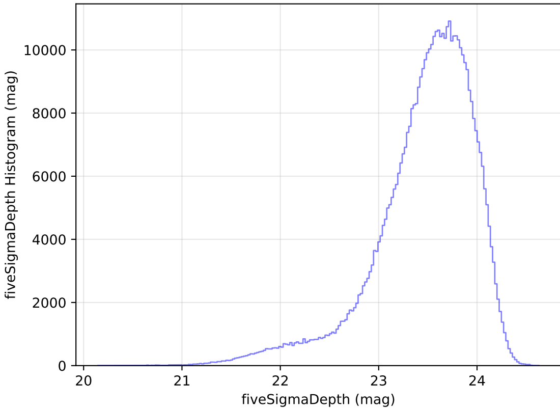
too_10_1v3.4_10yrs i: fiveSigmaDepth Histogram
