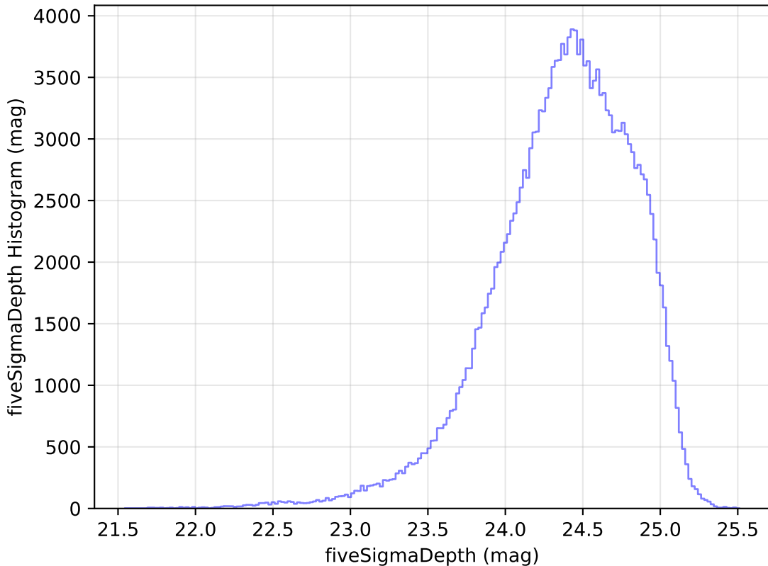
too_10_1v3.4_10yrs g: fiveSigmaDepth Histogram
