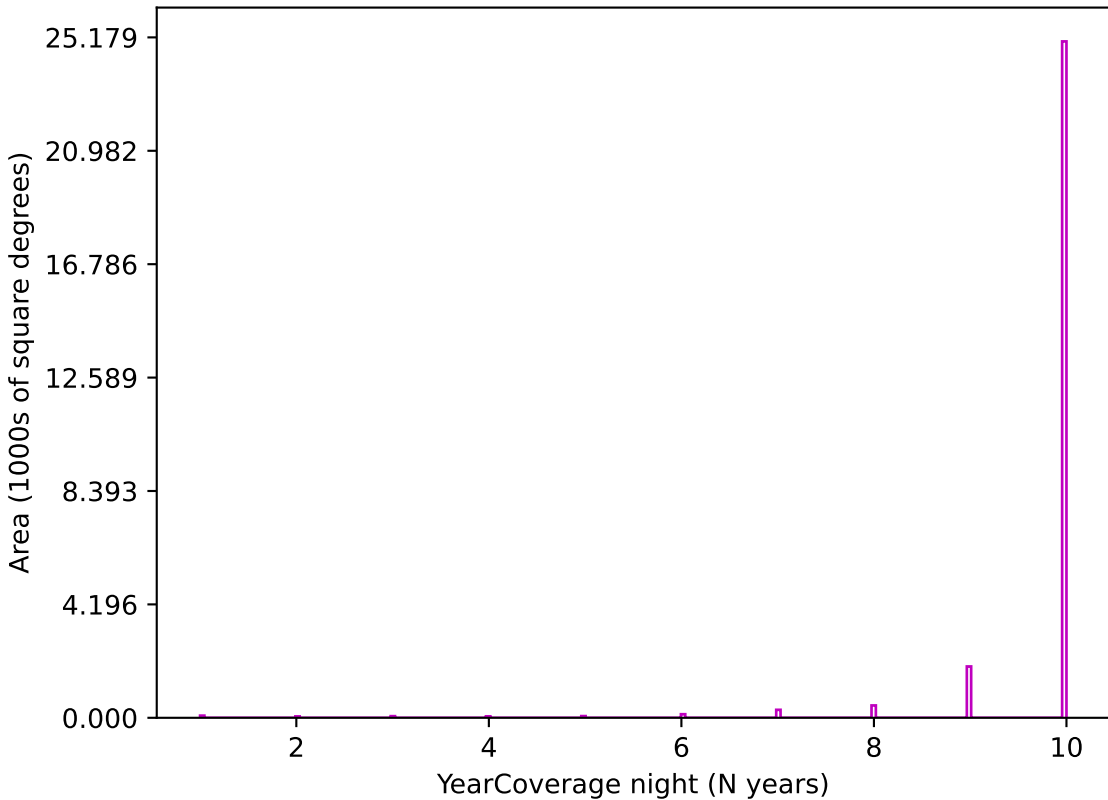
too_10_1v3.4_10yrs z band: YearCoverage night
