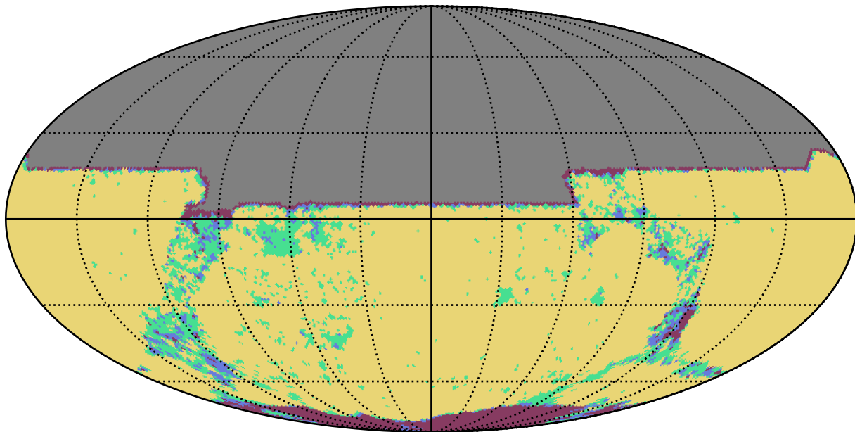
too_10_1v3.4_10yrs y band: YearCoverage night
