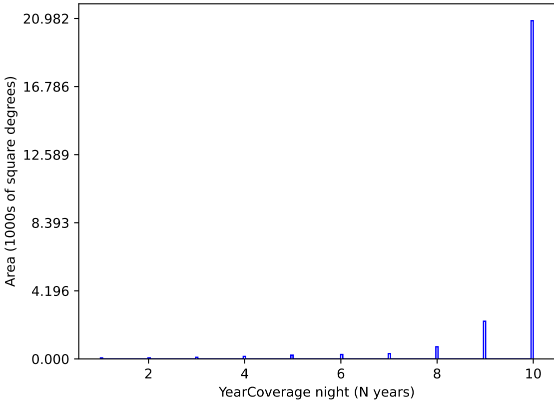
too_10_1v3.4_10yrs y band: YearCoverage night
