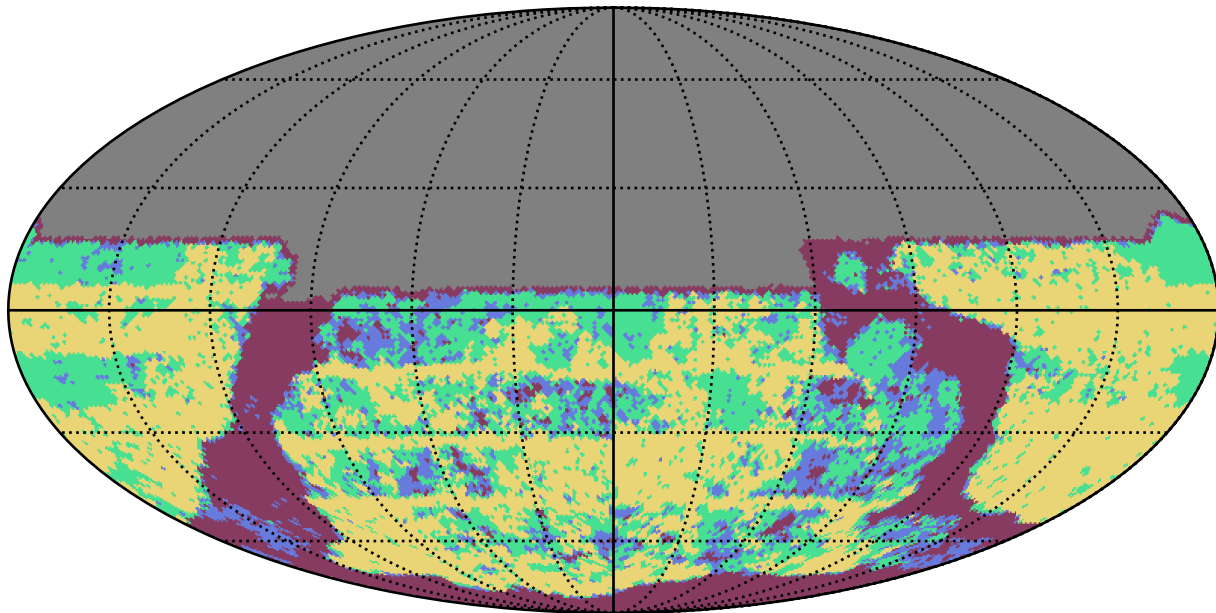
too_10_1v3.4_10yrs u band: YearCoverage night
