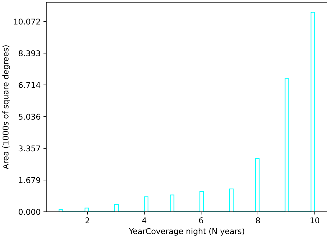
too_10_1v3.4_10yrs u band: YearCoverage night
