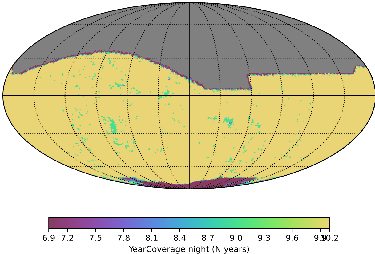
too_10_1v3.4_10yrs r band: YearCoverage night
