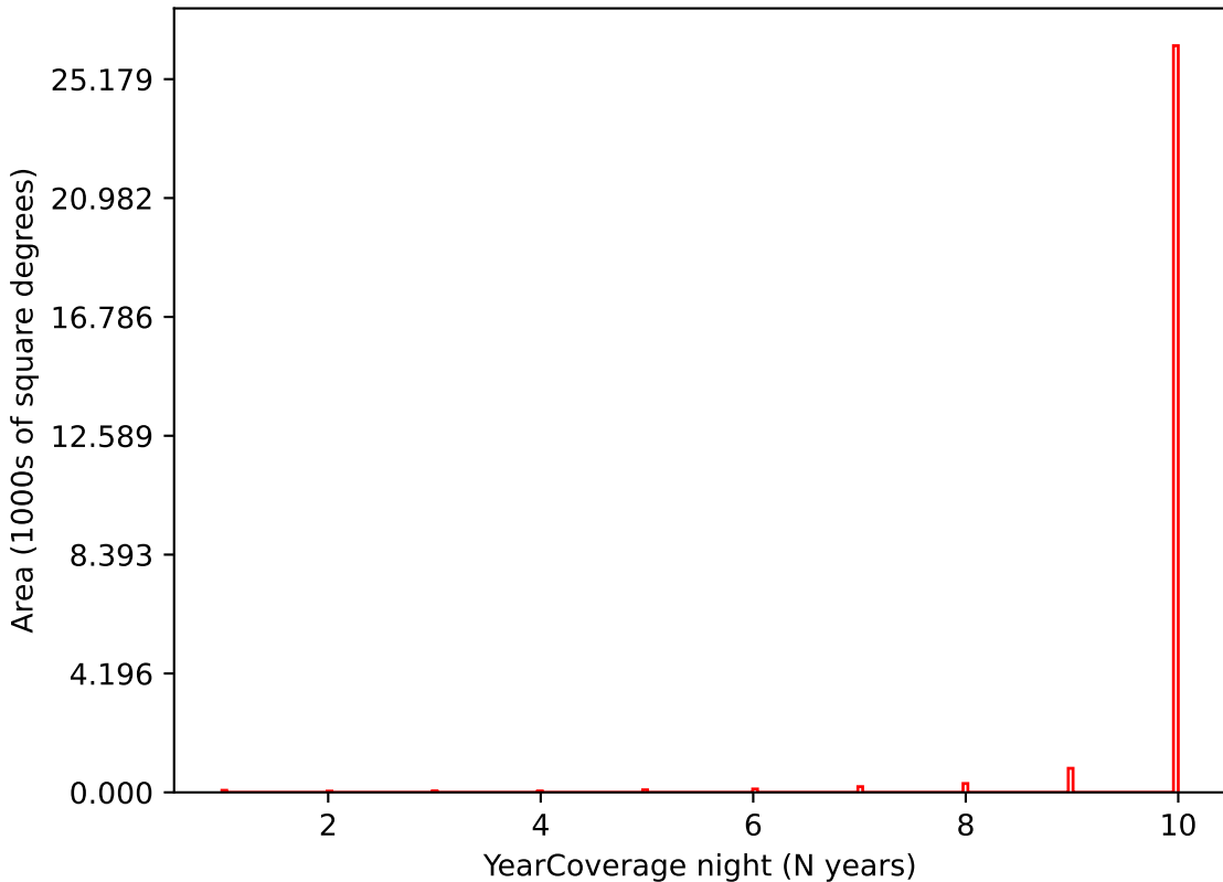
too_10_1v3.4_10yrs i band: YearCoverage night
