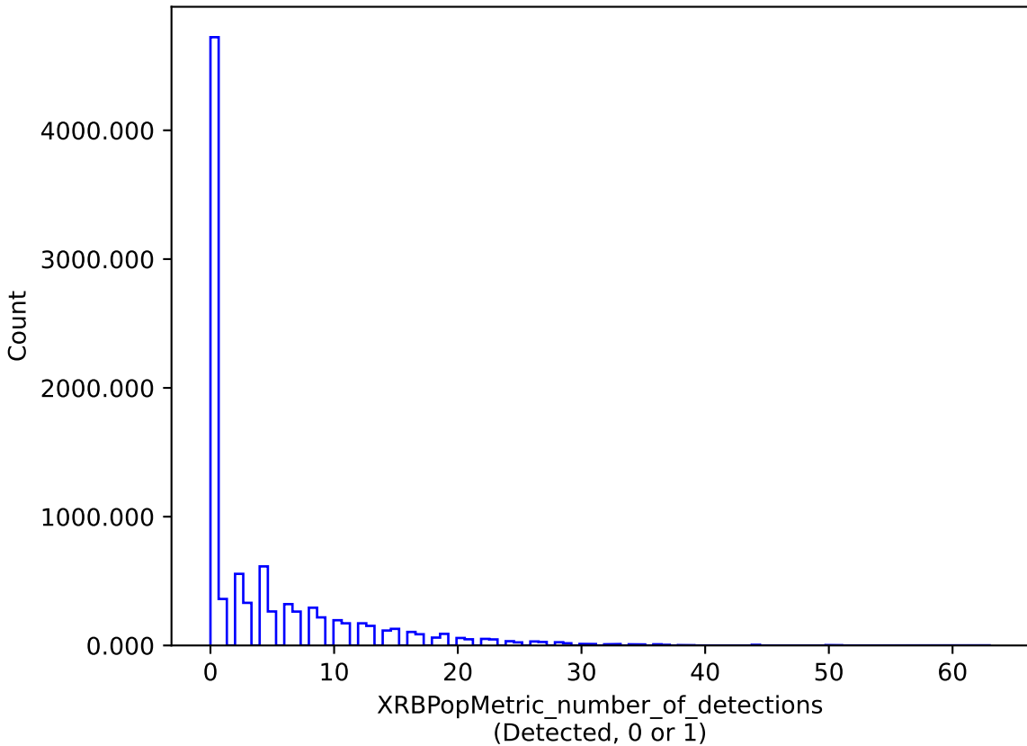
too_10_1v3.4_10yrs : XRBPoMetric_number_of_detections
