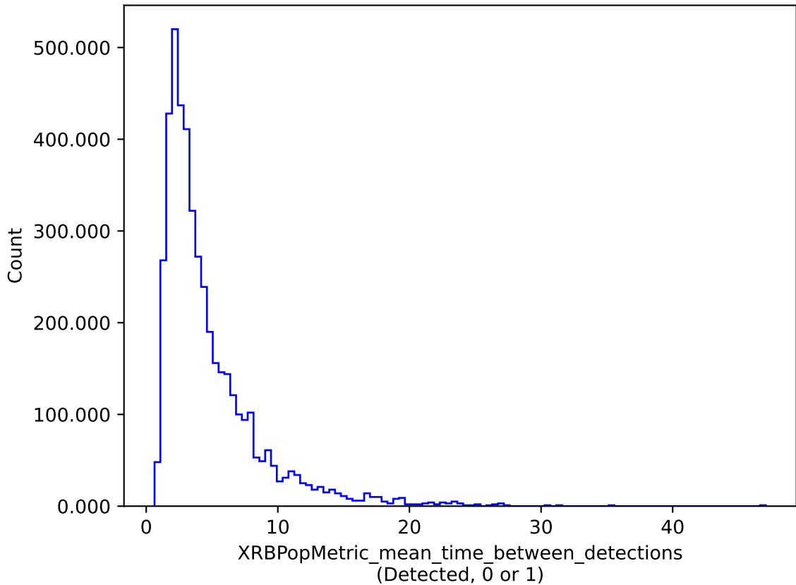
too_10_1v3.4_10yrs : XRBPoMetric_mean_time_between_detections
