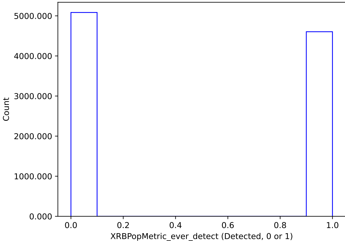
too_10_1v3.4_10yrs : XRBPoMetric_ever_detect
