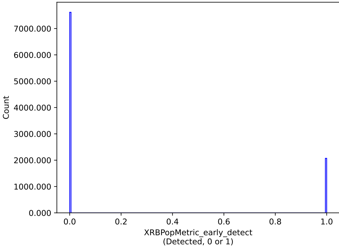
too_10_1v3.4_10yrs : XRBPoMetric_early_detect
