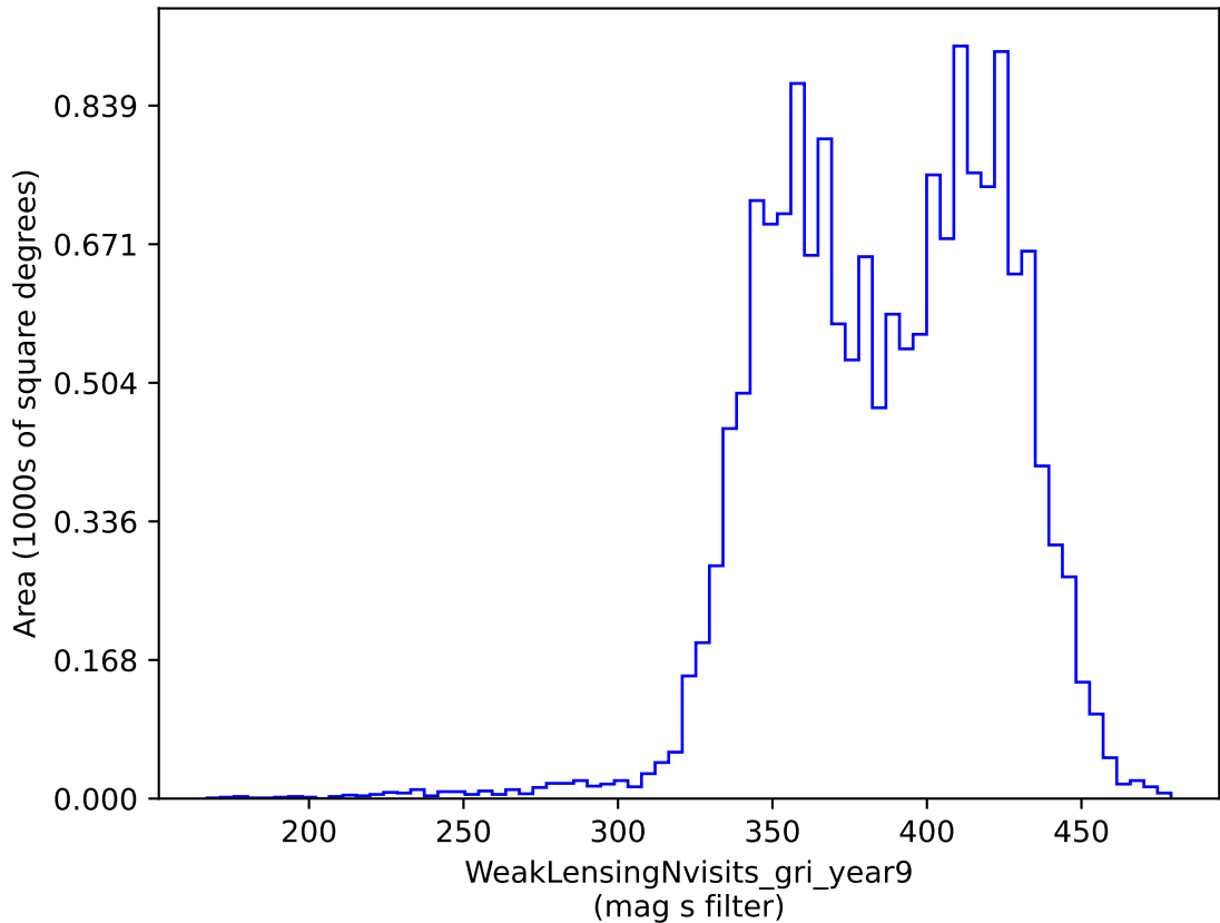
too_10_1v3.4_10yrs gri band non-DD: WeakLensingNvisits_gri_year9
