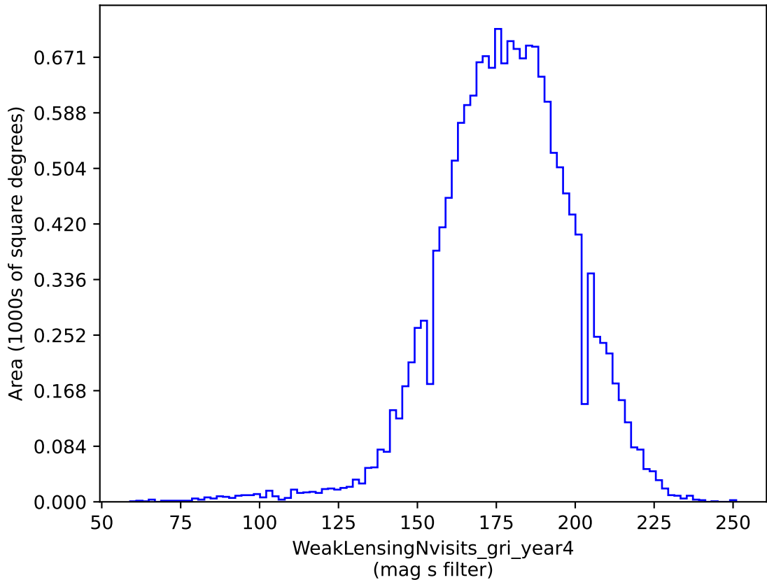
too_10_1v3.4_10yrs gri band non-DD: WeakLensingNvisits_gri_year4
