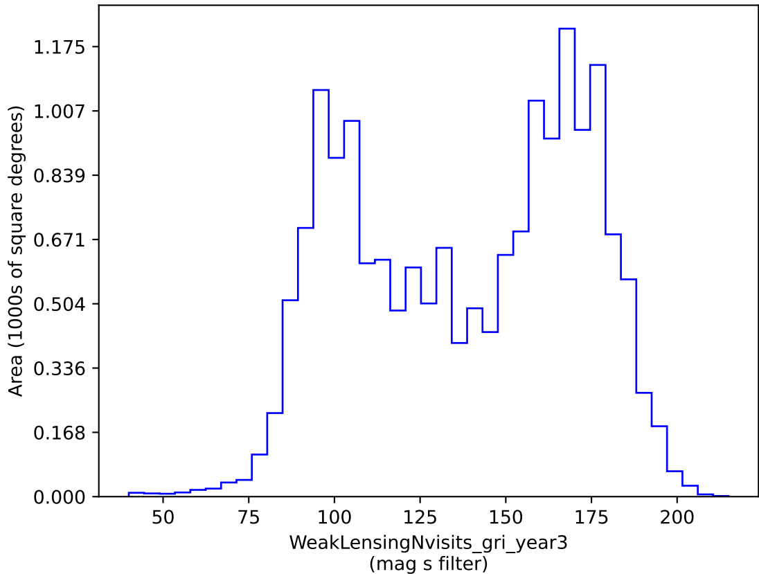
too_10_1v3.4_10yrs gri band non-DD: WeakLensingNvisits_gri_year3
