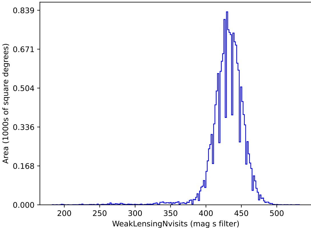
too_10_1v3.4_10yrs gri band non-DD: WeakLensingNvisits
