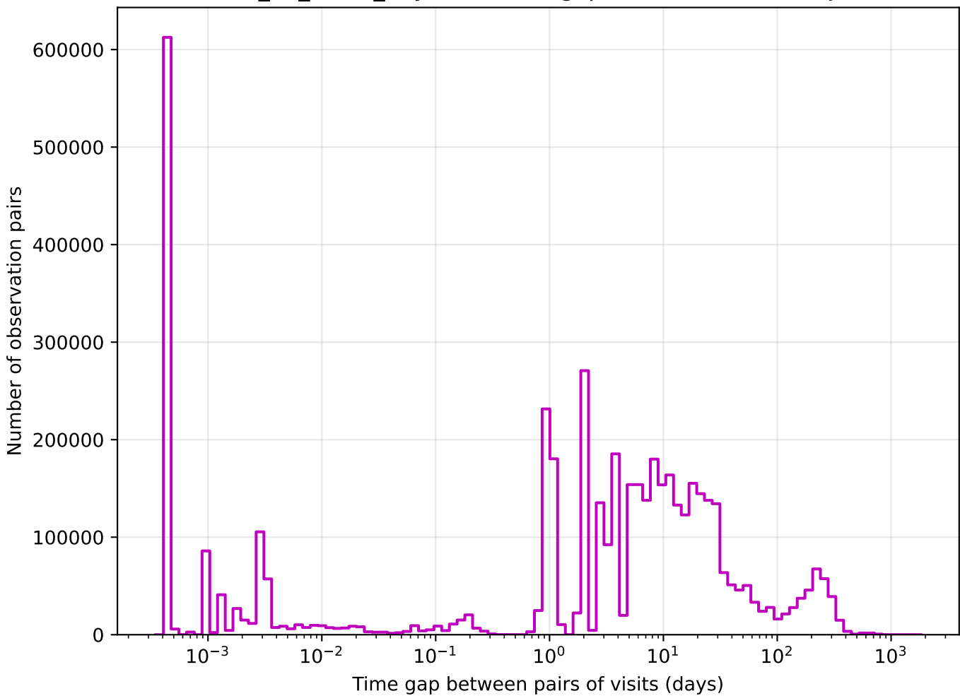
too_10_1v3.4_10yrs z band: Tgaps observationStartMJD
