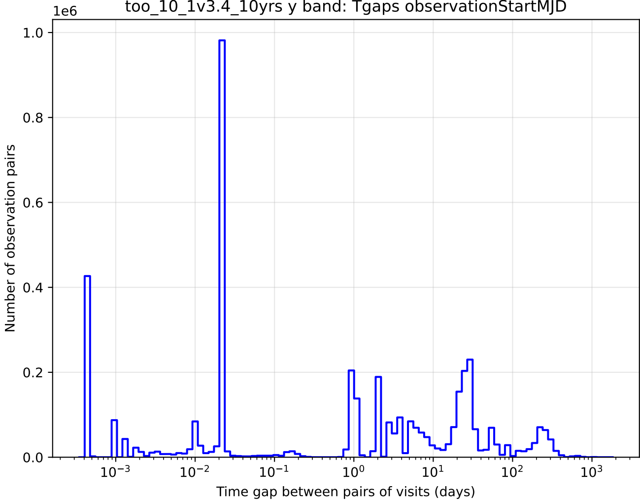
too_10_1v3.4_10yrs y band: Tgaps observationStartMJD
