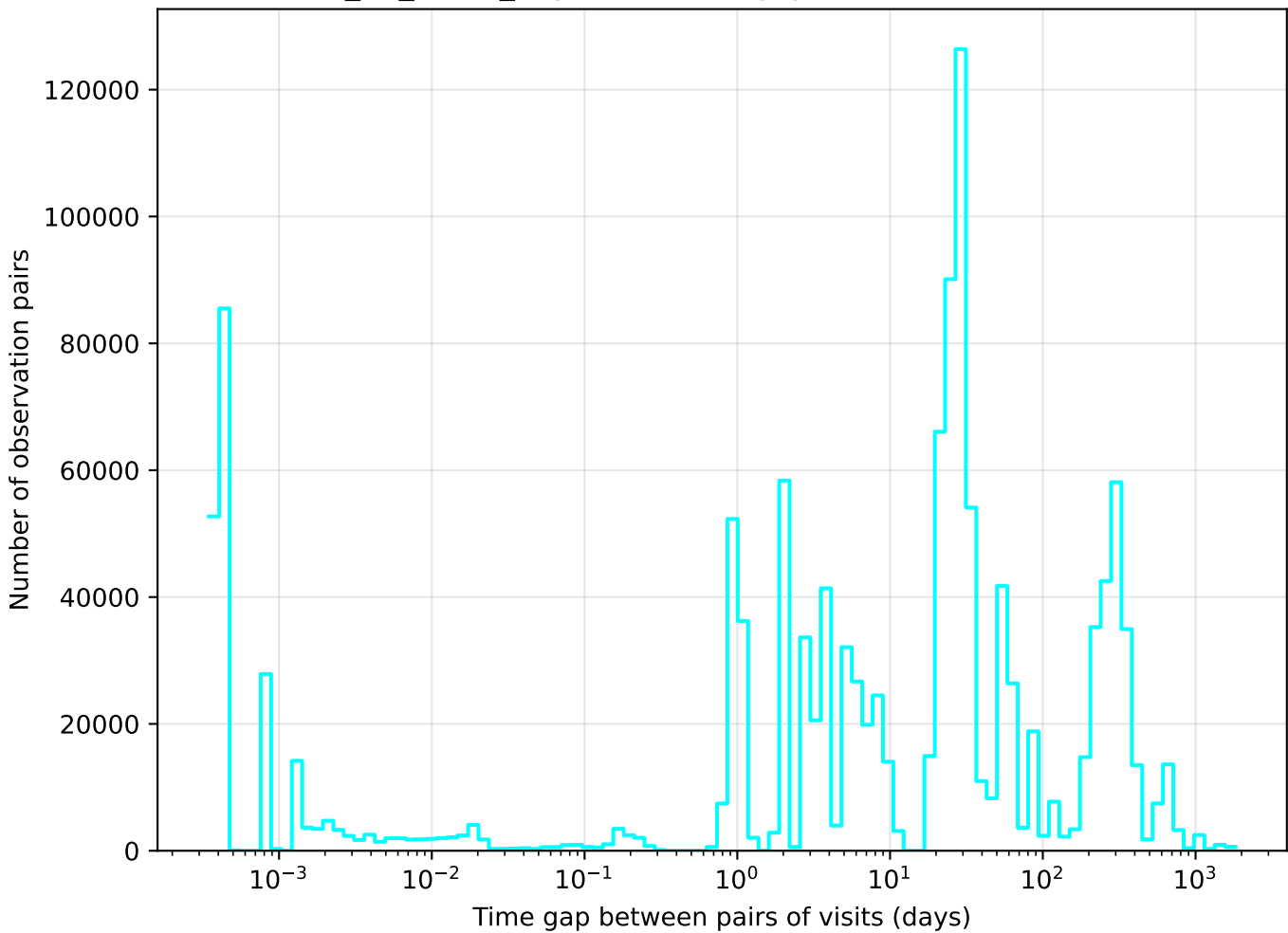
too_10_1v3.4_10yrs u band: Tgaps observationStartMJD
