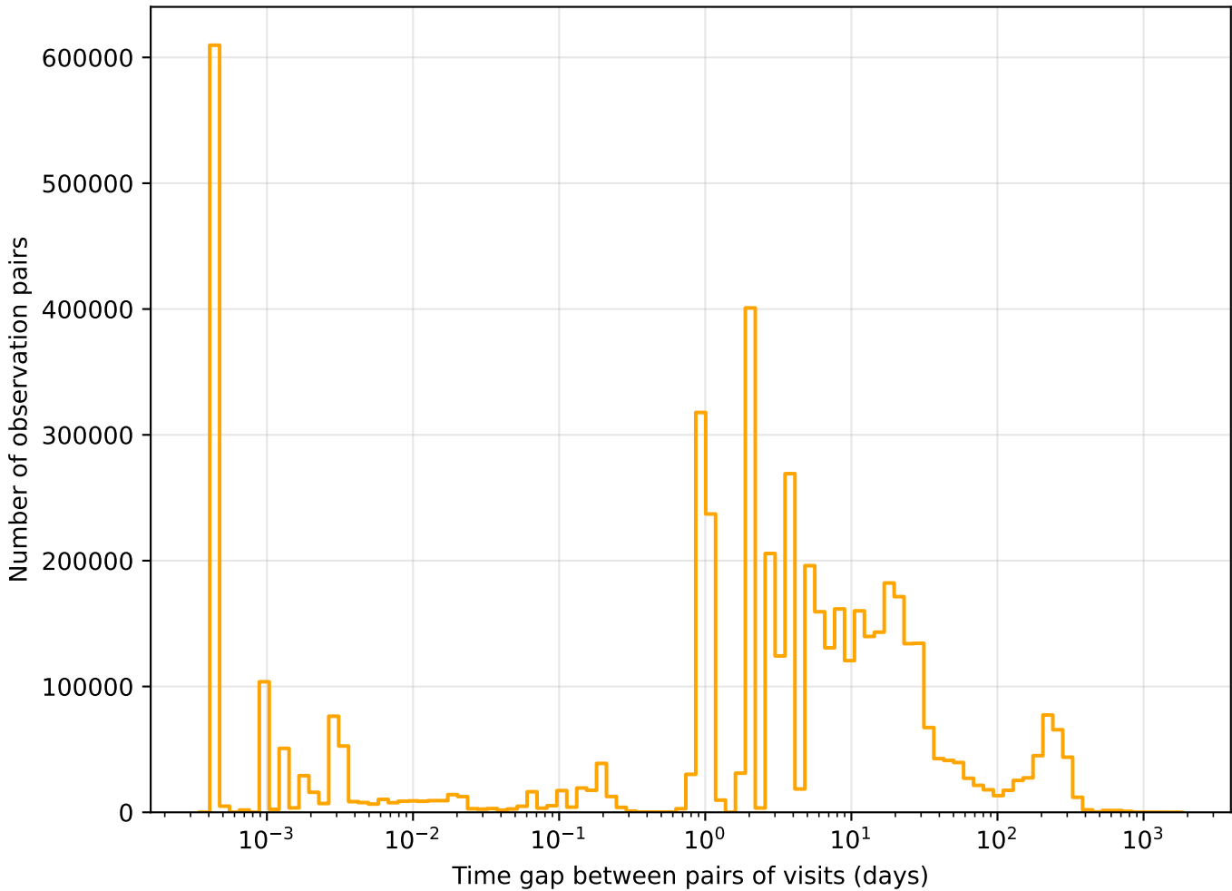
too_10_1v3.4_10yrs r band: Tgaps observationStartMJD
