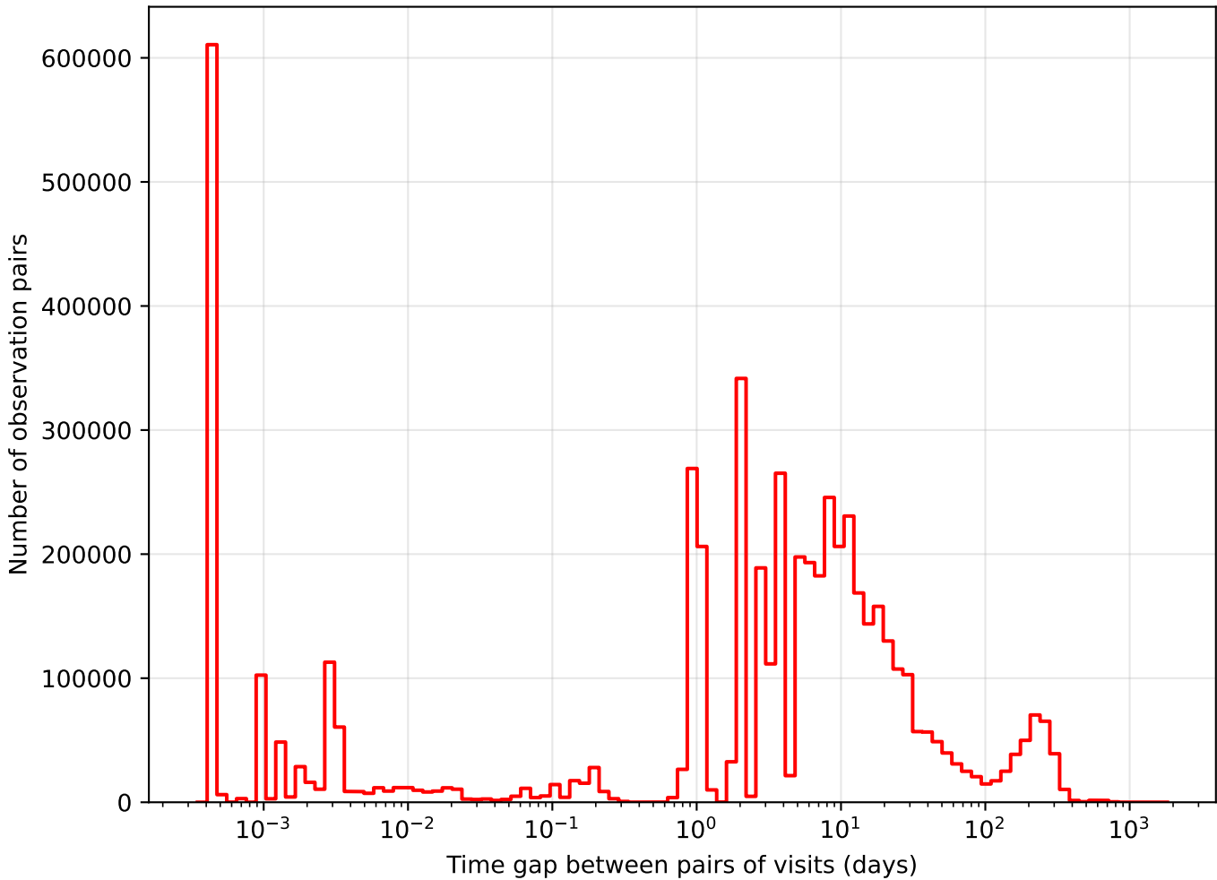
too_10_1v3.4_10yrs i band: Tgaps observationStartMJD
