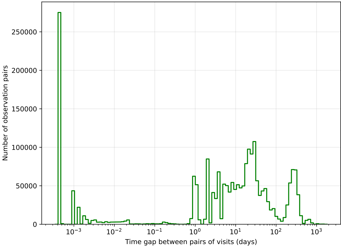
too_10_1v3.4_10yrs g band: Tgaps observationStartMJD
