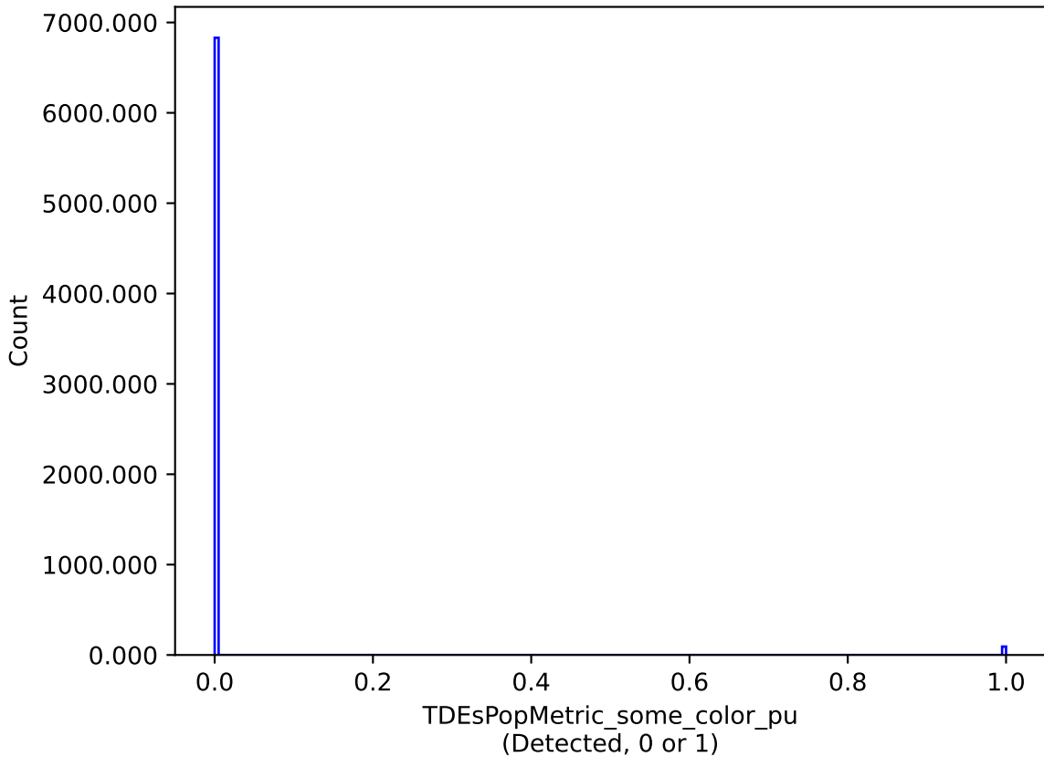
too_10_1v3.4_10yrs : TDEsPopMetric_some_color_pu
