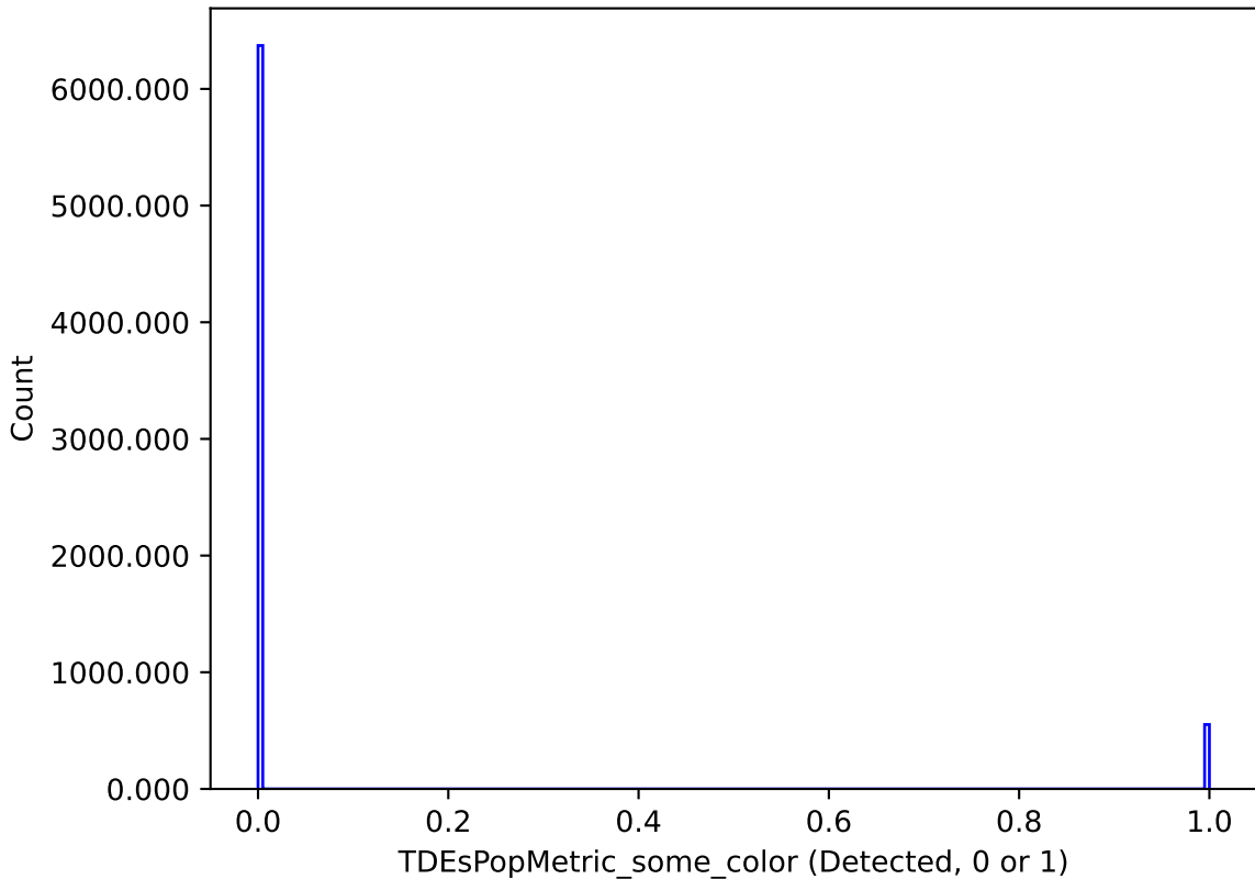
too_10_1v3.4_10yrs : TDEsPopMetric_some_color
