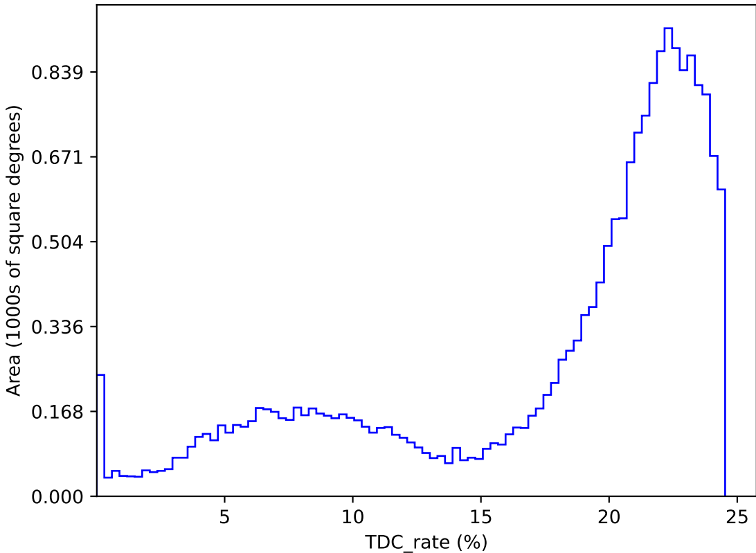
too_10_1v3.4_10yrs : TDC_rate
