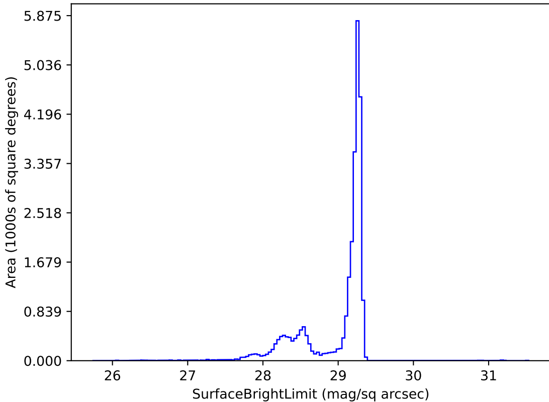
too_10_1v3.4_10yrs z: SurfaceBrightLimit
