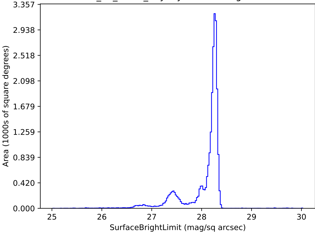
too_10_1v3.4_10yrs y: SurfaceBrightLimit
