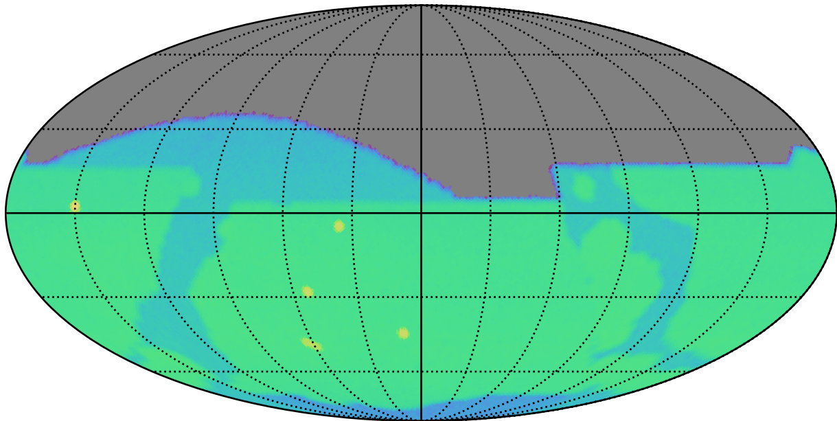
too_10_1v3.4_10yrs r: SurfaceBrightLimit
